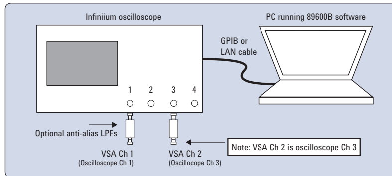
Figure 1b. Equipment connections for 4-channel oscilloscopes used to provide 2-channel input to 89600B VSA software 1
