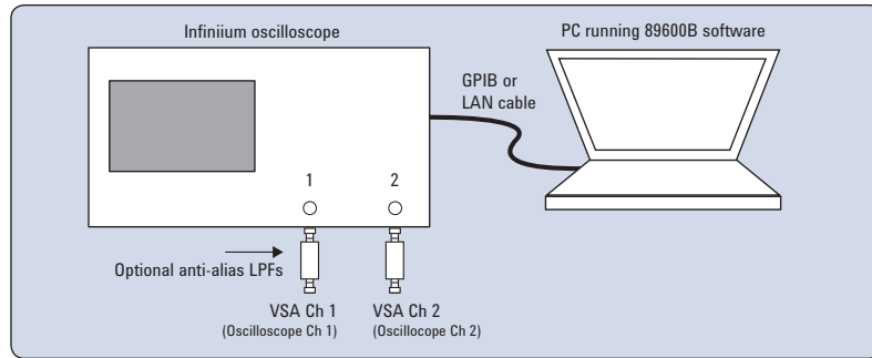
Figure 1a. Equipment connections for 2-channel oscilloscopes 1
