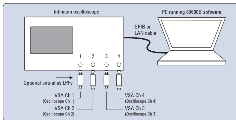
Figure 1c. Equipment connections for 4-channel oscilloscopes used to provide 3- or 4-channel VSA measurements using the 89600B VSA software 1
